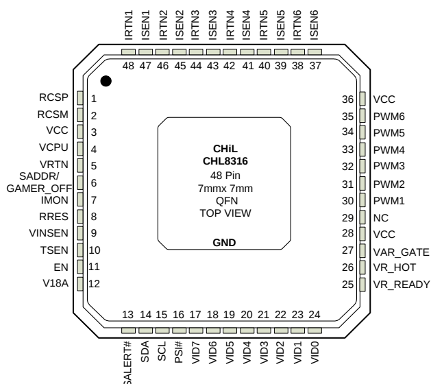
Figure 1. CHL8316 48 Pin QFN Package
