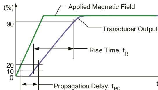
Figure 2: Propagation Delay and Rise Time Definitions
