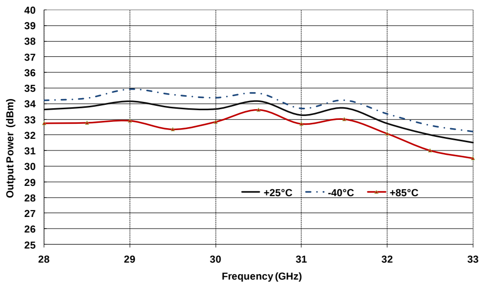
Output Power versus Frequency &amp; Temperature
