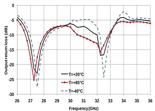
Output return loss versus Frequency &amp; Temperature
