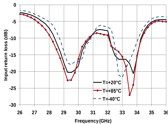
Input Return Loss versus Frequency &amp; Temperature
