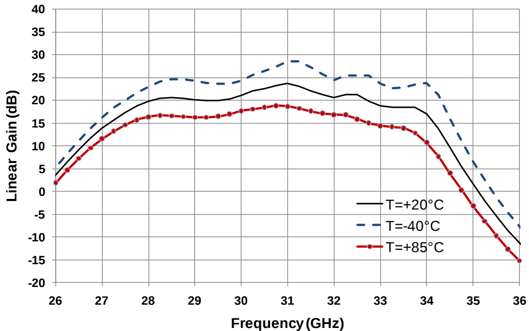
Linear gain versus Frequency &amp; Temperature
