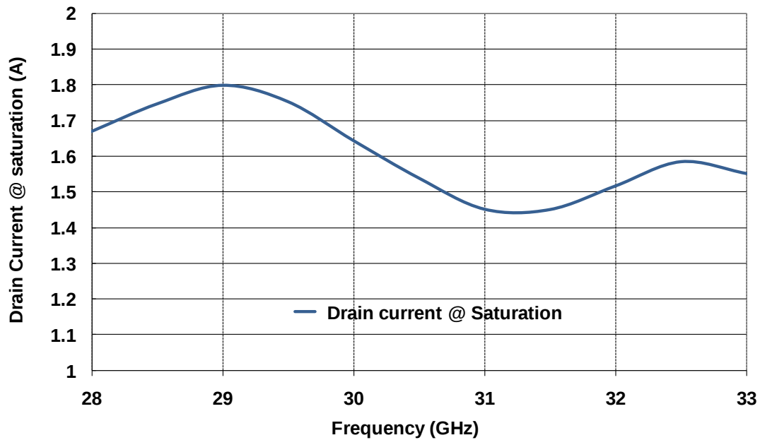
Drain current @ saturation versus Frequency
