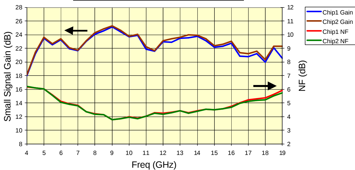
CHA6518 : Noise Figure @ 25°C
