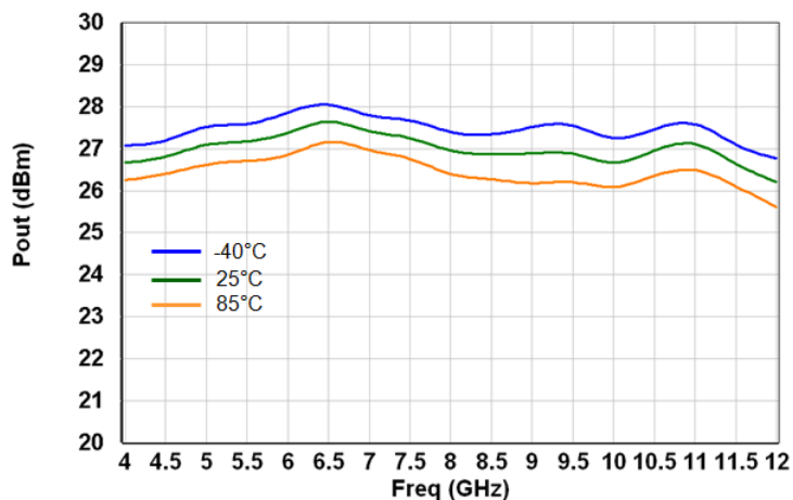
Output power at 3dB gain compression
