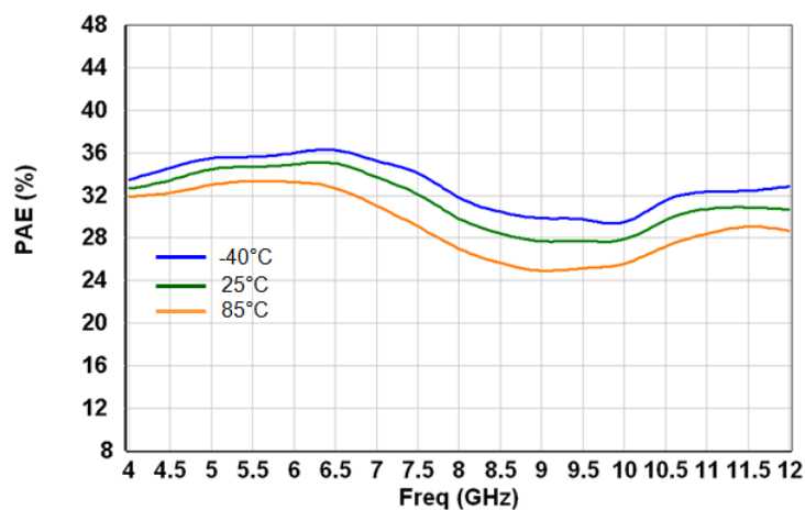
PAE at 1dB gain compression
