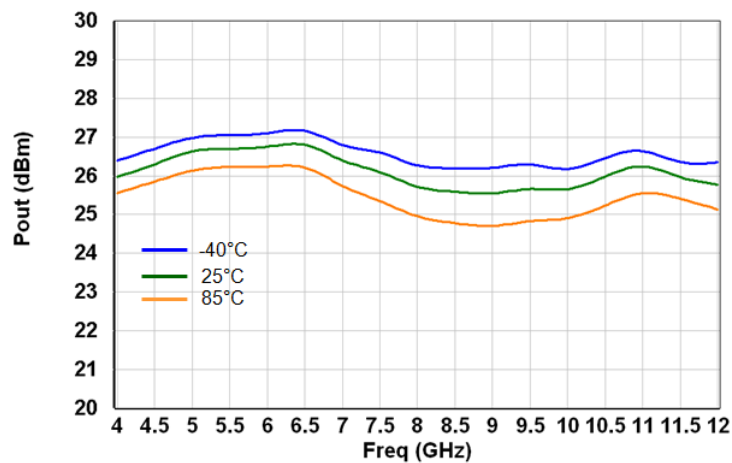
Output power at 1dB gain compression
