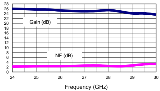
Typical on wafer measurements : Gain & NF
