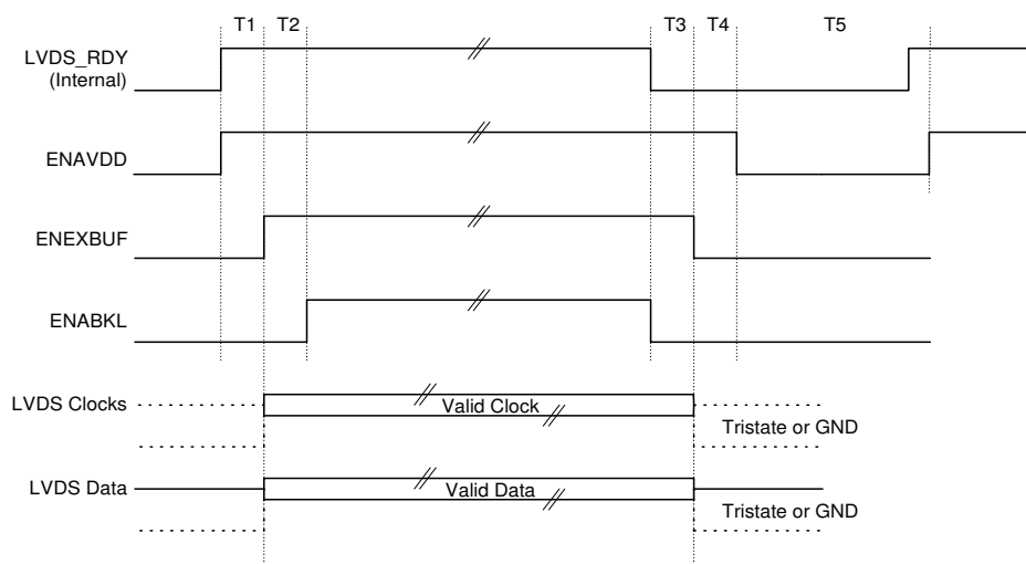
Figure 5: Power Sequencing
