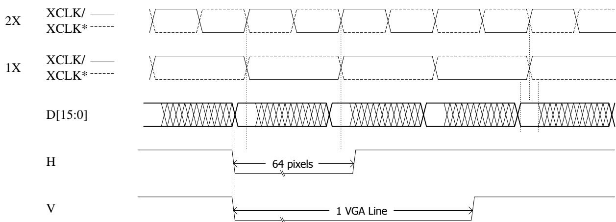
Figure 3: Clock, Data and Interface Timing
