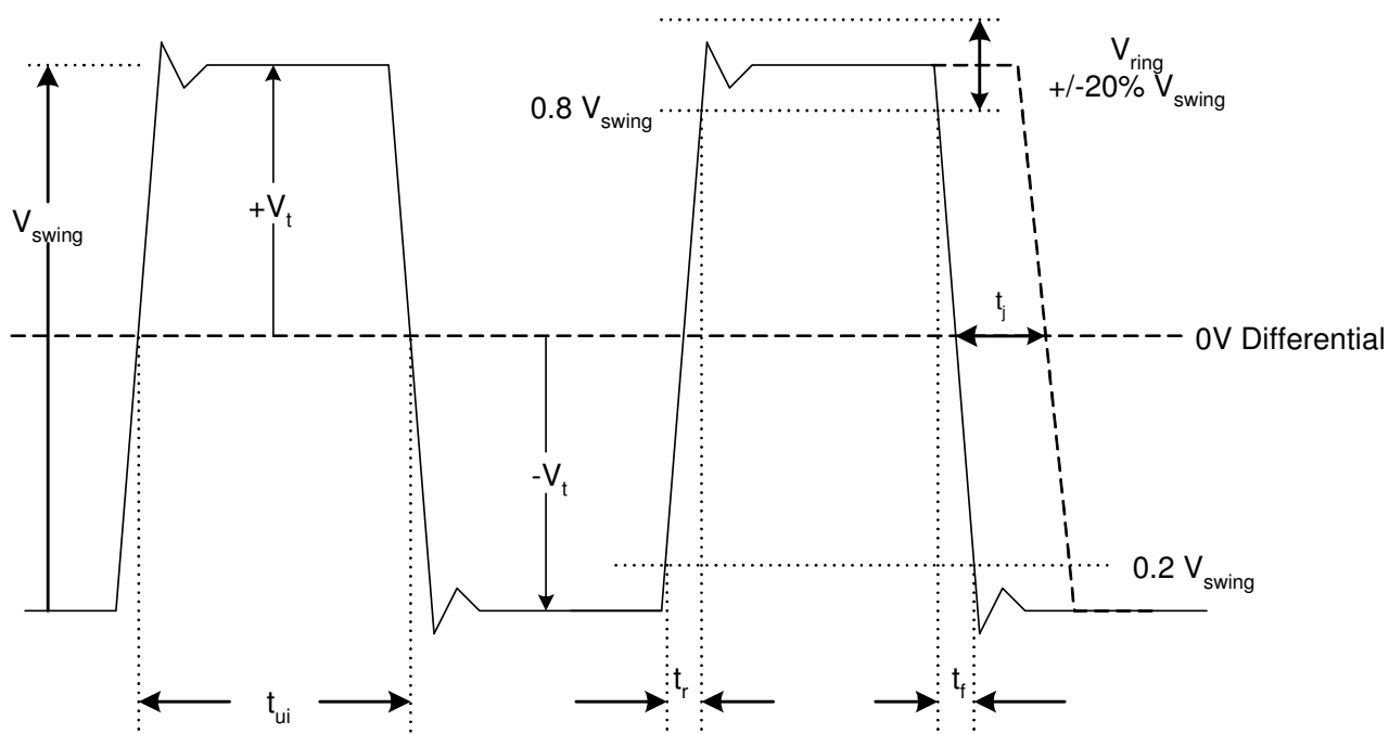
Figure 7: AC Timing for LVDS Outputs
