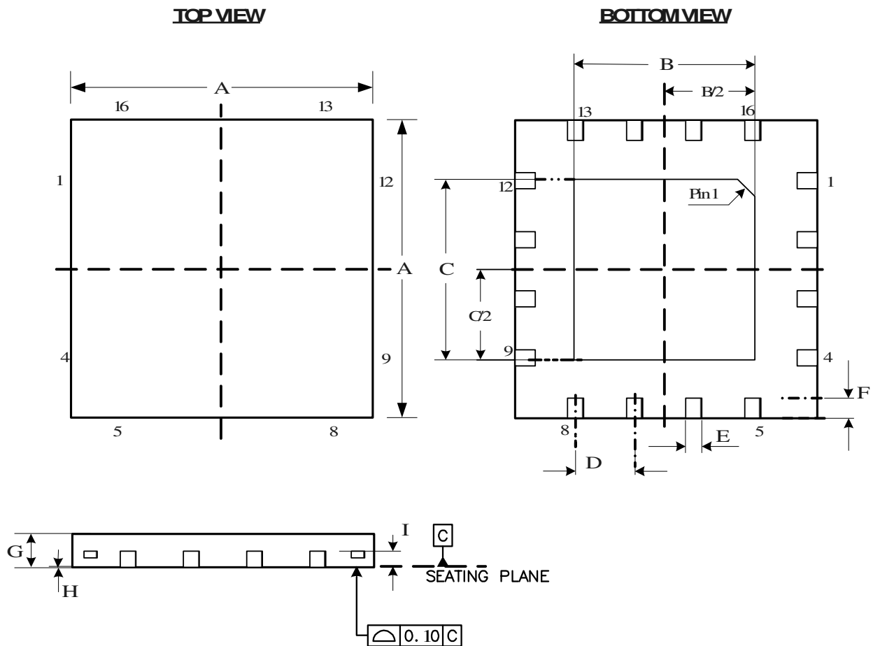
16 Pin QFN Package (3 x 3 mm)
