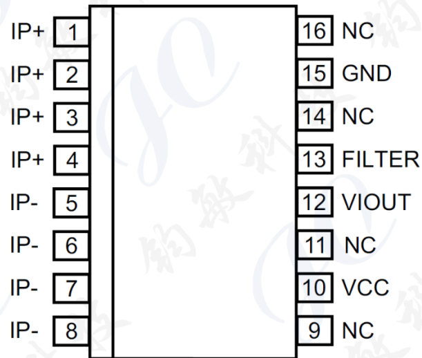
Pinout Diagram
