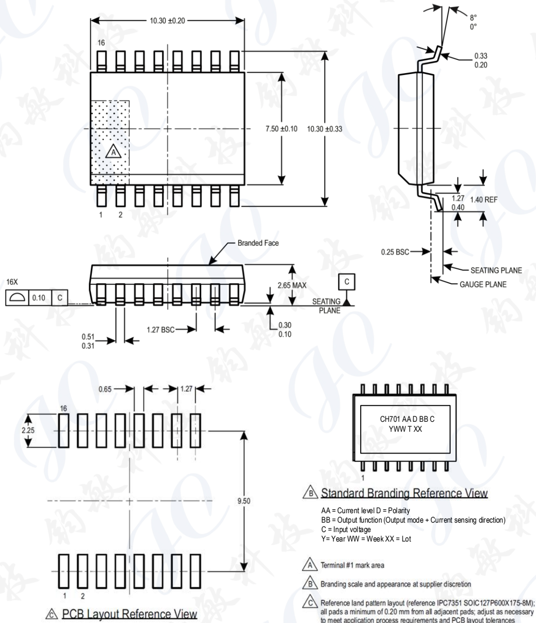
Figure 7: Package SOW16
