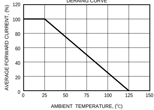
FIG. 4 - TYPICAL FORWARD CURRENT DERAING CURVE
