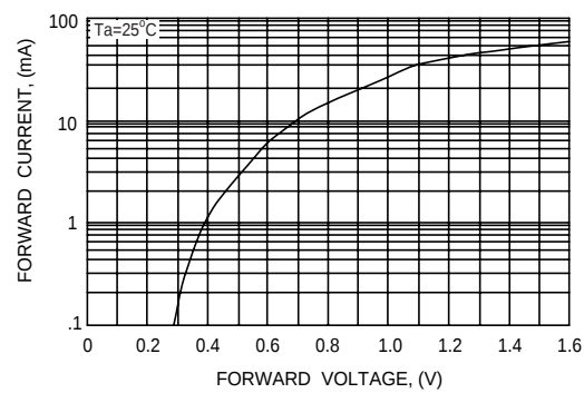
FIG. 2 - FORWARD CHARACTERISTICS
