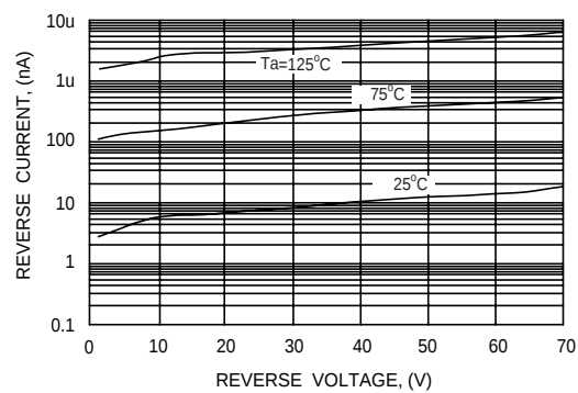
FIG. 3 - REVERSE CHARACTERISTICS
