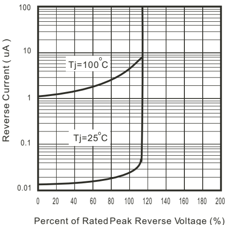
Fig. 1 - Reverse Characteristics
