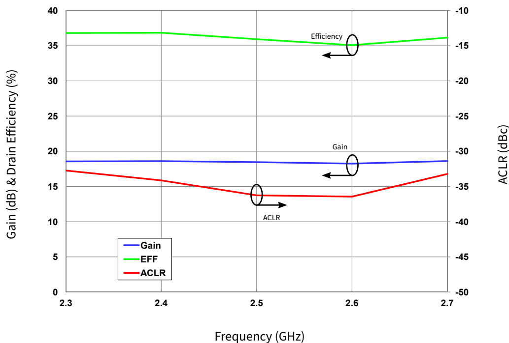
Figure 6. Typical Gain, Drain Efficiency and ACLR vs Frequency
