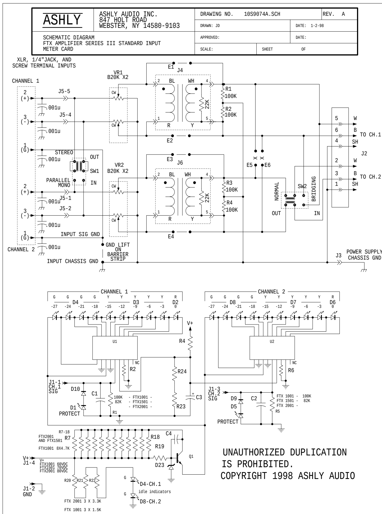
Figure 15.3: FTX Power Amplifier Standard Input and Meter
