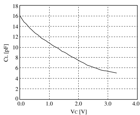
V_{DD} = 3.3V
