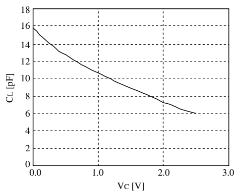
V_{DD} = 2.5V
