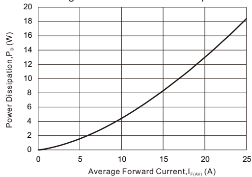
Fig. 3 - Forward Power Dissipation
