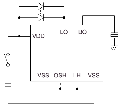
Circuit 2
