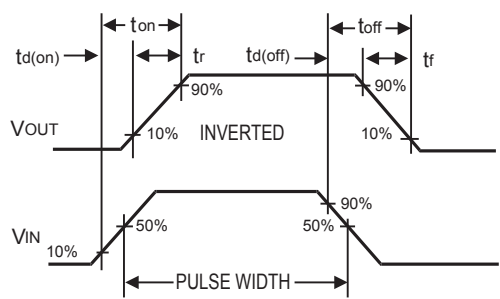
Figure 10. Switching Waveforms
