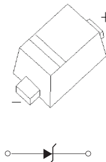
SOD-723
