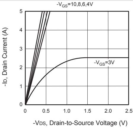
Figure 1. Output Characteristics
