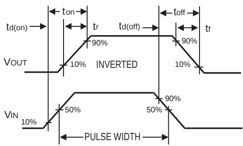
Figure 18. Switching Waveforms
