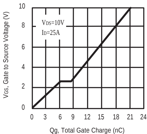
Figure 9. Gate Charge
