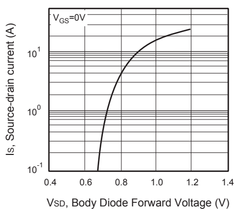
Figure 4. Body Diode Forward Voltage Variation with Source Current
