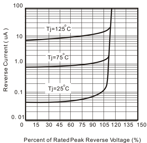
Fig. 1 - Reverse Characteristics
