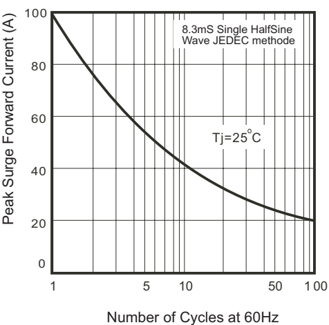
Fig. 4 - Non Repetitive Forward Surge Current
