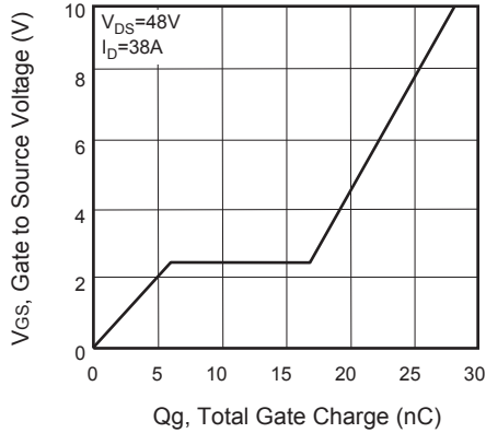
Figure 7. Gate Charge
