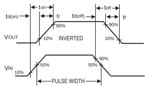
Figure 10. Switching Waveforms
