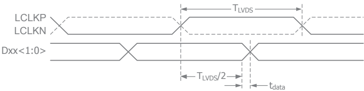
Figure 4. Data Timing
