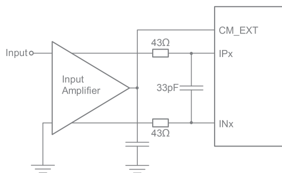
Figure 9. DC-Coupled Input
