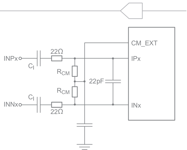
Figure 11. AC-Coupled Input
