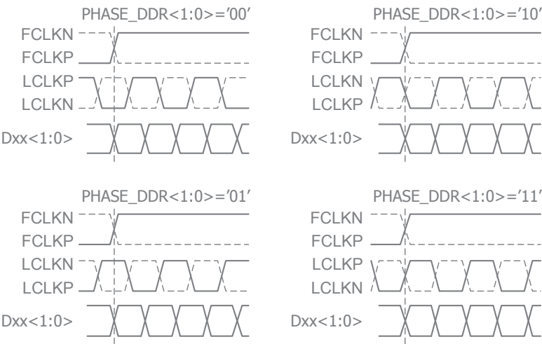
Figure 6. Phase Programmability Modes for LCLK
