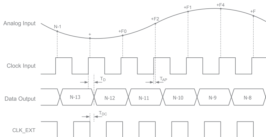
Figure 1. Timing Diagram
