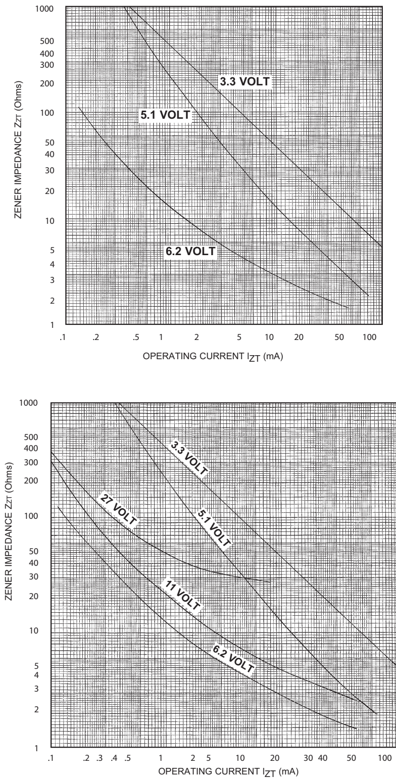
ZENER IMPEDANCE VS. OPERATING CURRENT
