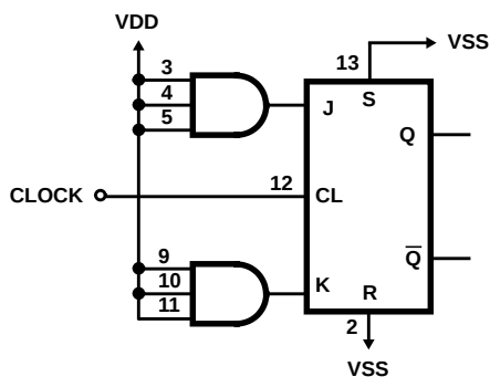
FIGURE 4. CD4095BMS CONNECTED IN TOGGLE MODE
