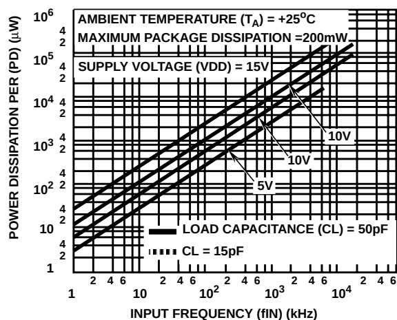
FIGURE 14. TYPICAL POWER DISSIPATION vs INPUT CLOCK FREQUENCY
