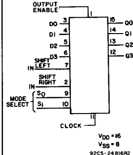
4-Bit Bidirectional Universal Shift Register
