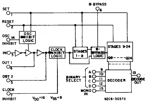
Programmable Timer
