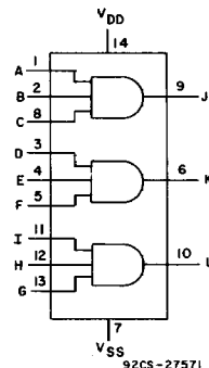
Triple 3-Input AND Gate
