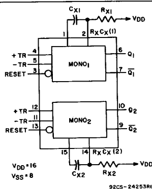
Dual Precision Monostable Multivibrator
