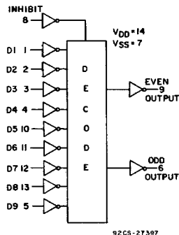
9-Bit Parity Generator/Checker
