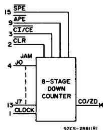
8-Stage Presettable Synchronous Down Counter
