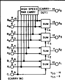
4-Bit Full Adder with Parallel Carry Out
