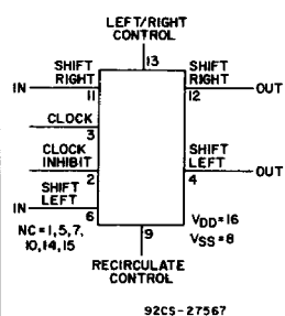
32-Stage Static Left/Right Shift Register
