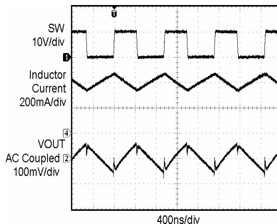
Switching Waveform
