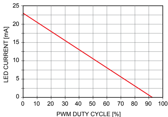
Figure 3. Filtered PWM Dimming [0V to 2.5V]
