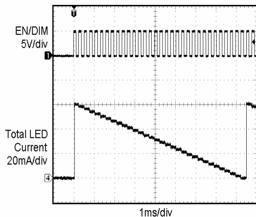
Dimming Waveform
