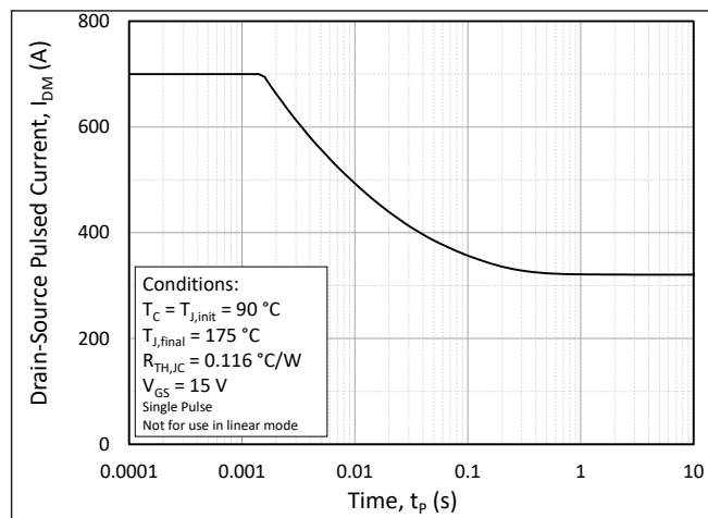
Figure 20. Pulsed Current Safe Operating Area
