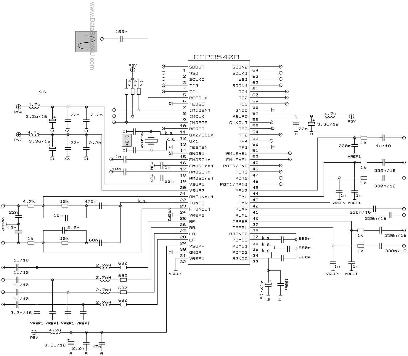
Fig. 7-1: Typical Application Circuit
