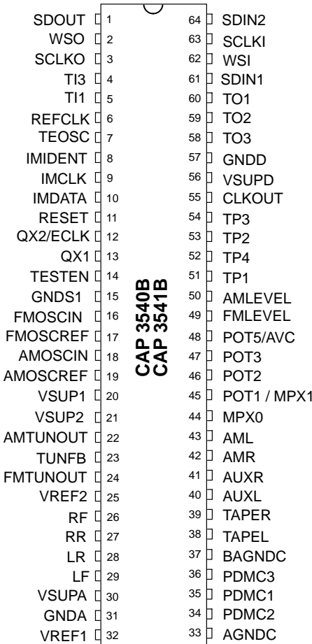
Fig. 3–4: Pinning of the CAP 3540B in PSDIP64 package, top view MPLEVEL not available ERR not available POT4 not available TI2 not available (internally pushed to GND)
