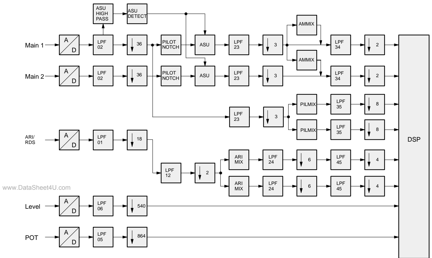
Fig. 2-5: Digital signal processing blocks, input side
