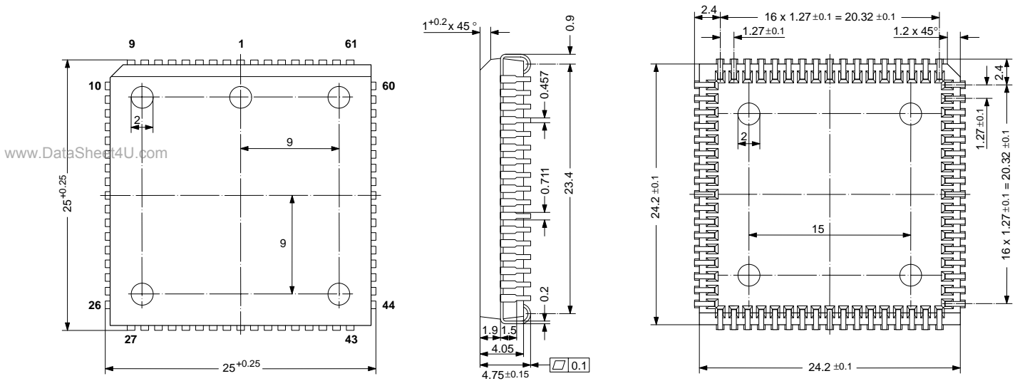
Fig. 3-2: 68-Pin Plastic Leaded Chip Carrier Package (PLCC68) Weight approximately 4.8 g Dimensions in mm
