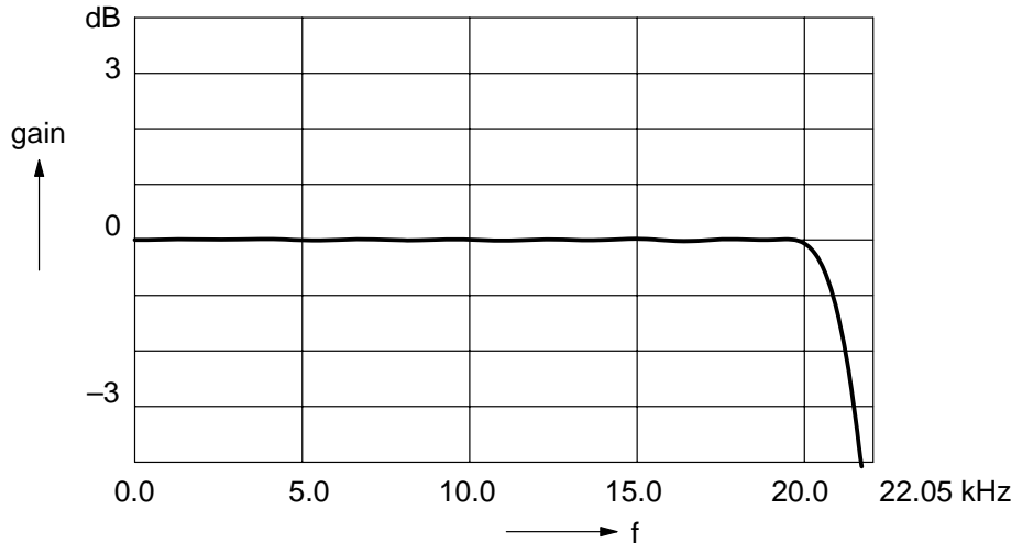
Fig. 2-10: Digital interpolation filter, passband characteristic
