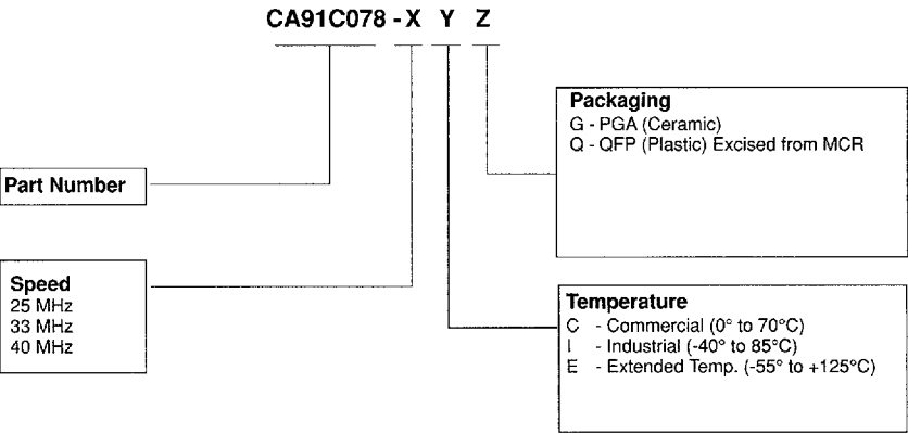
Valid Suffixes for CA91C078
