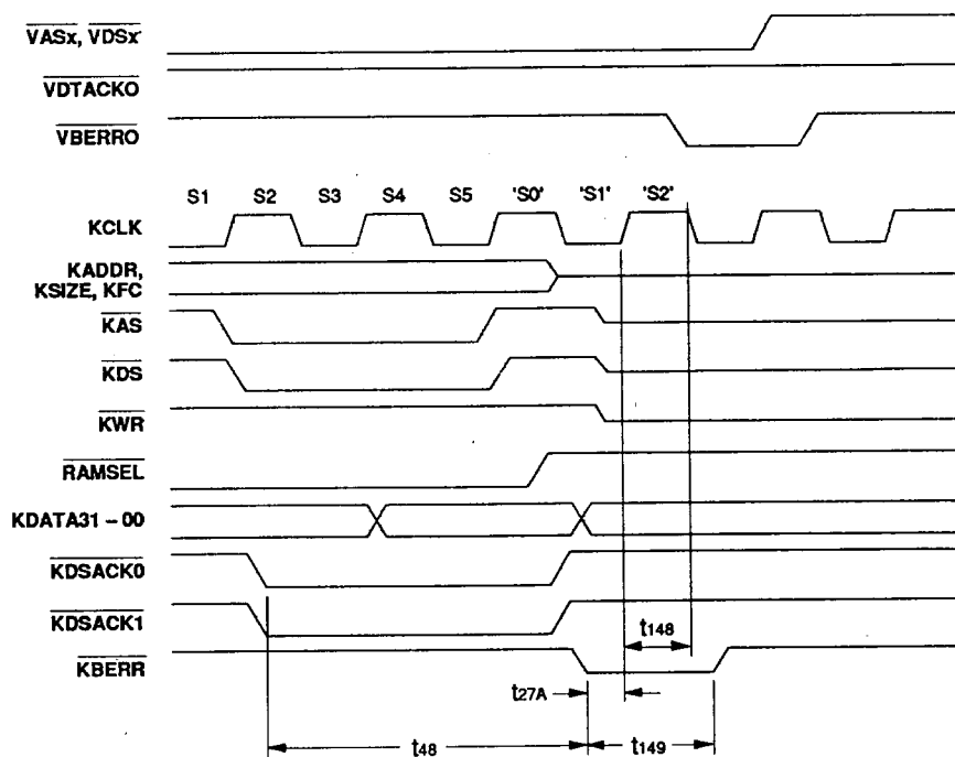
Figure 18b : DART SLAVE INTERFACE, MEMORY READ with LATE KBERR
