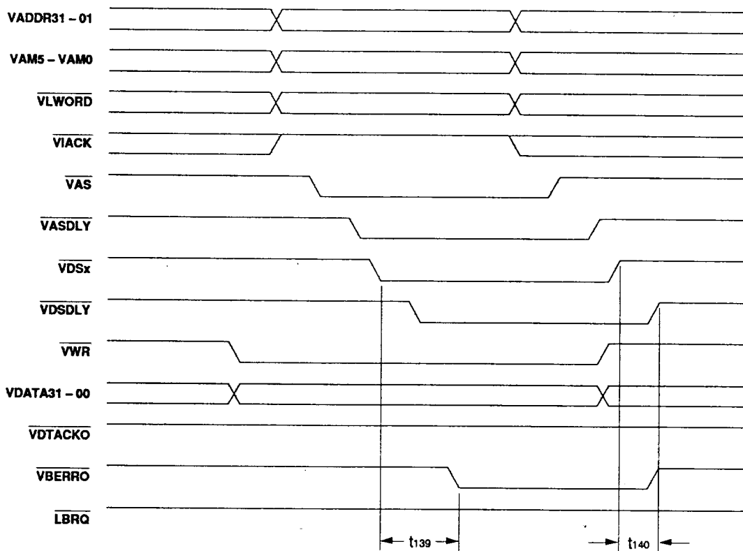
Figure 20 : DARF VME SLAVE INTERFACE, ILLEGAL ACCESS
