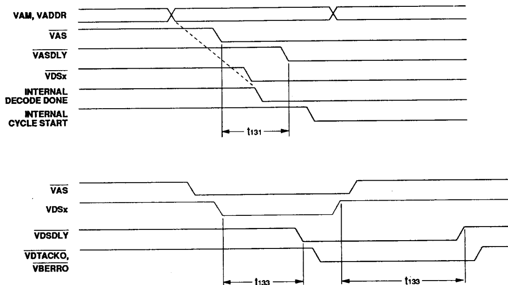
Figure 21 : DARF DELAY LINE TIMING, VMEbus SLAVE CYCLES
