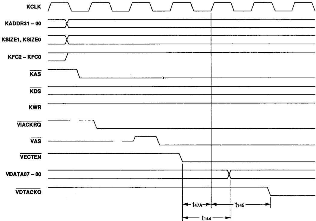
Figure 14 : DART MASTER INTERFACE, VMEbus Iack CYCLE
