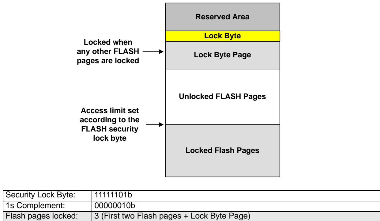
Figure 15.1. Flash Program Memory Map
