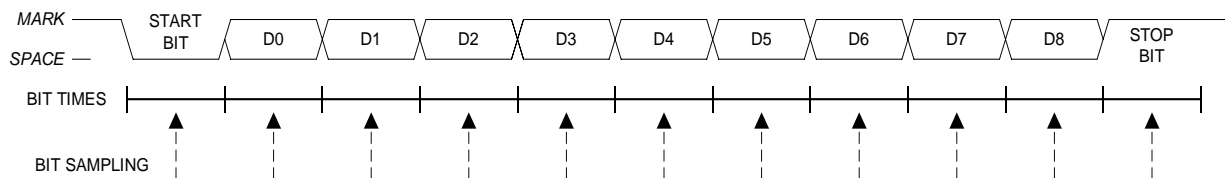
Figure 21.5. UART0 Modes 2 and 3 Timing Diagram
