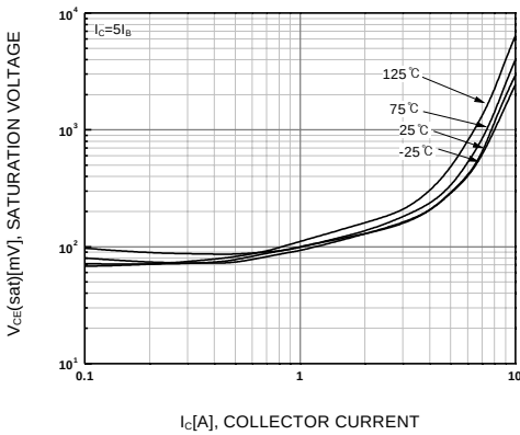
Figure 5. Collector-Emitter Saturation Voltage 2
