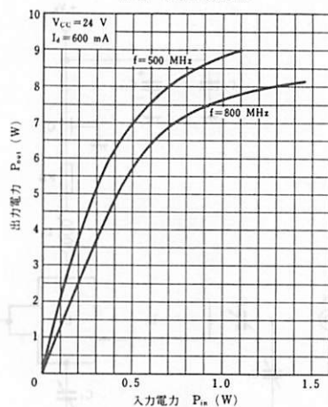
OUTPUT POWER vs. INPUT POWER (class A)
