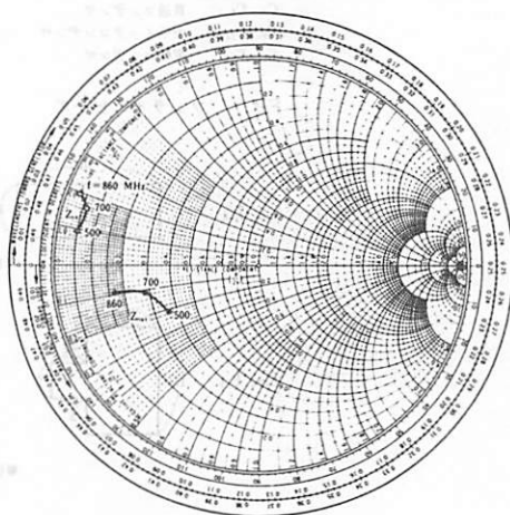
Z_{in} , Z_{out} Data (class A)
