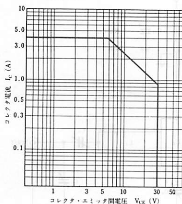
FORWARD BIAS SAFE OPERATING AREA (DC)
