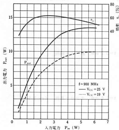
OUTPUT POWER, COLLECTOR EFFICIENCY vs. INPUT POWER (class C)
