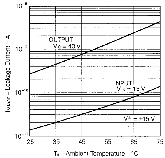
LEAKAGE CURRENTS
