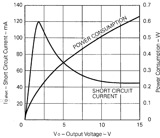
OUTPUT LIMITING CHARACTERISTICS
