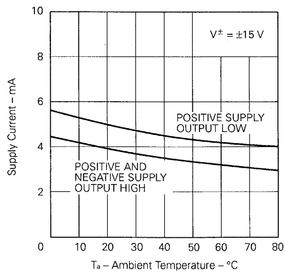
SUPPLY CURRENT
