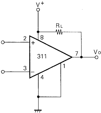
OPEN COLLECTOR OUTPUT
