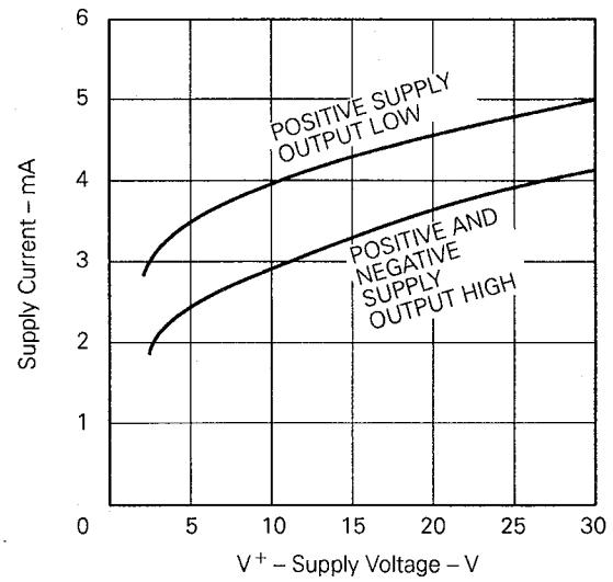
SUPPLY CURRENT
