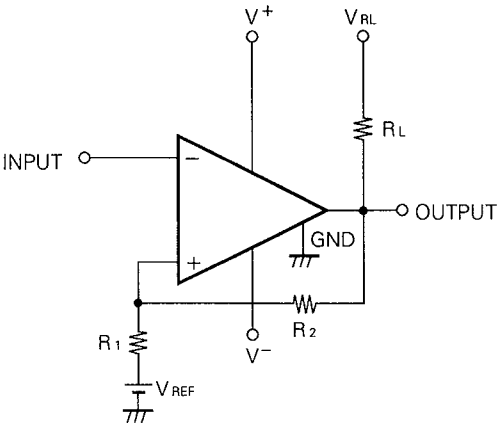
COMPARATOR with HYSTERESIS CIRCUIT
