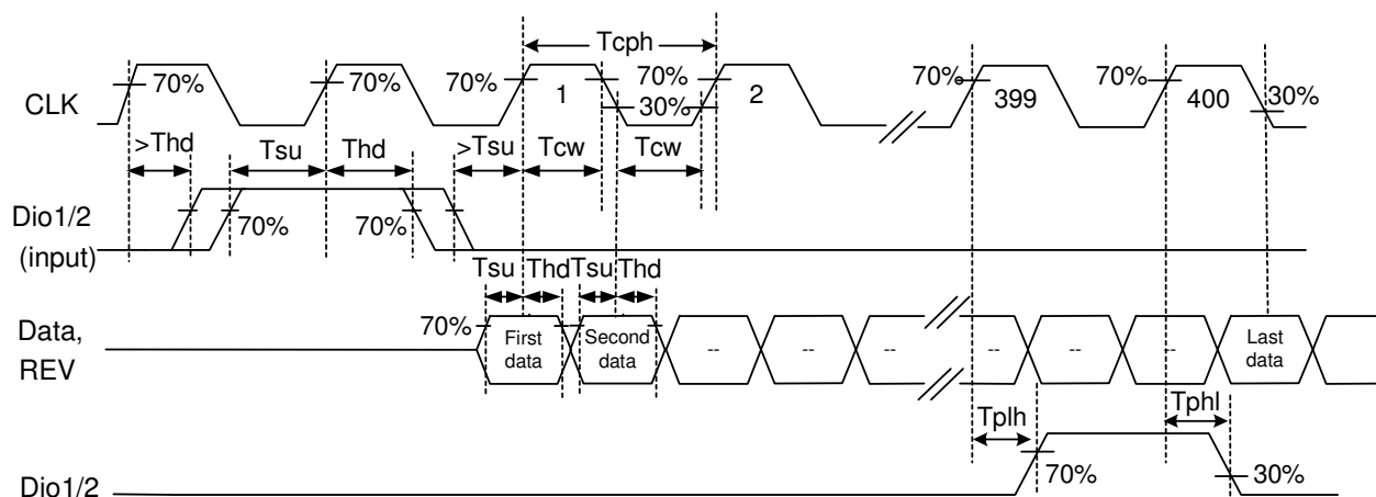
Timing Diagram 2
