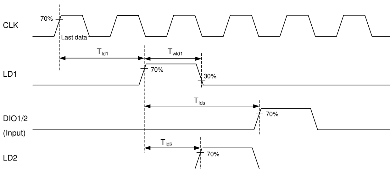
LD1 Timing Chart
