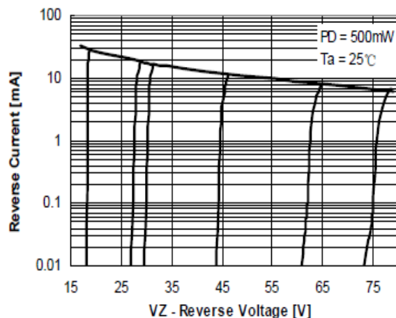
Figure 6. Reverse Current vs. Reverse Voltage
