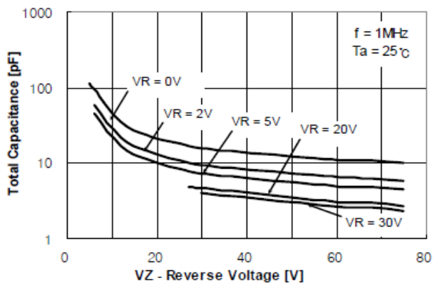
Figure 2. Total Capacitance
