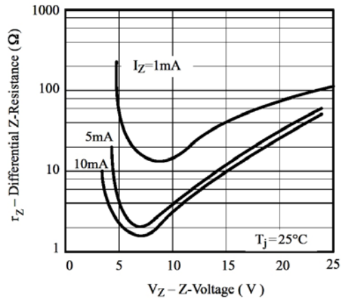
Figure 10. Differential Z-Resistance Vz vs. Z-Voltage
