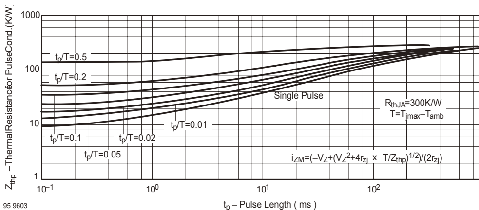
Fig.11 Thermal Response
