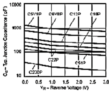
Figure 3. Typ. Diode Capacitance vs. Reverse Voltage
