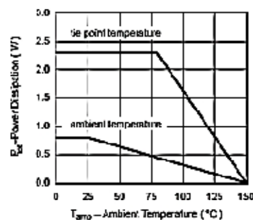
Figure 5. Power Dissipation vs. Ambient Temperature
