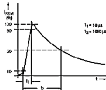
Figure 4. Non-Repetitive Peak Reverse Current Pulse Definition
