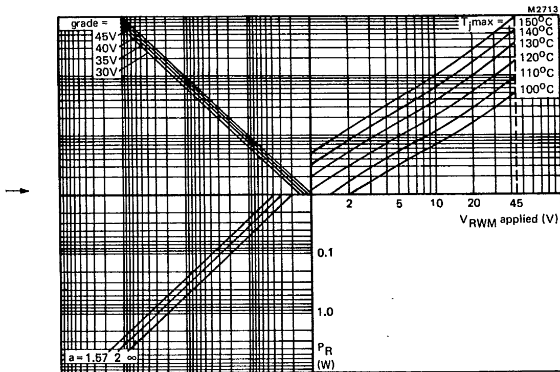
Fig.5 NOMOGRAM: for calculation of P_R (reverse leakage power dissipation) for a given T_j \text{ max.} , V_{RWM} applied, voltage grade and form factor. a = \text{form factor} = I_F(\text{RMS})/I_F(\text{AV}) .
