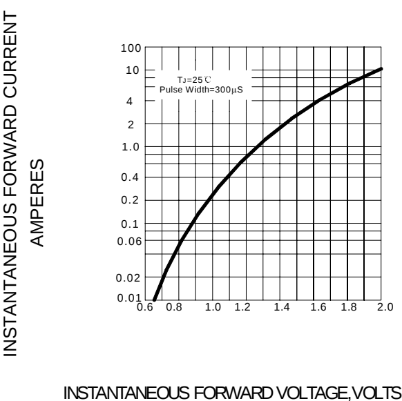
FIG.4-TYPICAL FORWARD CHARACTERISTIC
