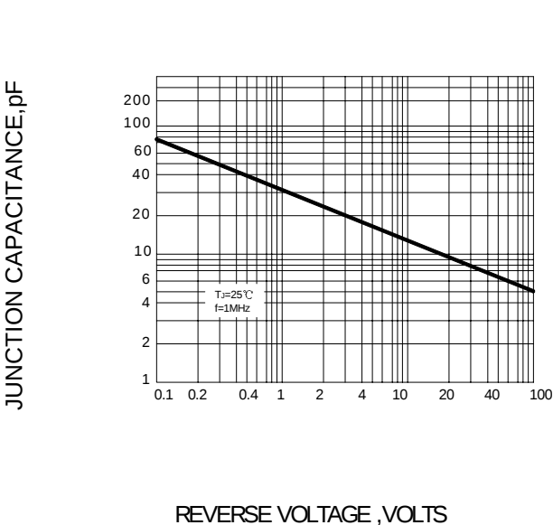
FIG.5-TYPICAL JUNCTION CAPACITANCE
